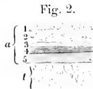
Section of top of mound facing the Roy, half a mile north of its junction with the Turret.
